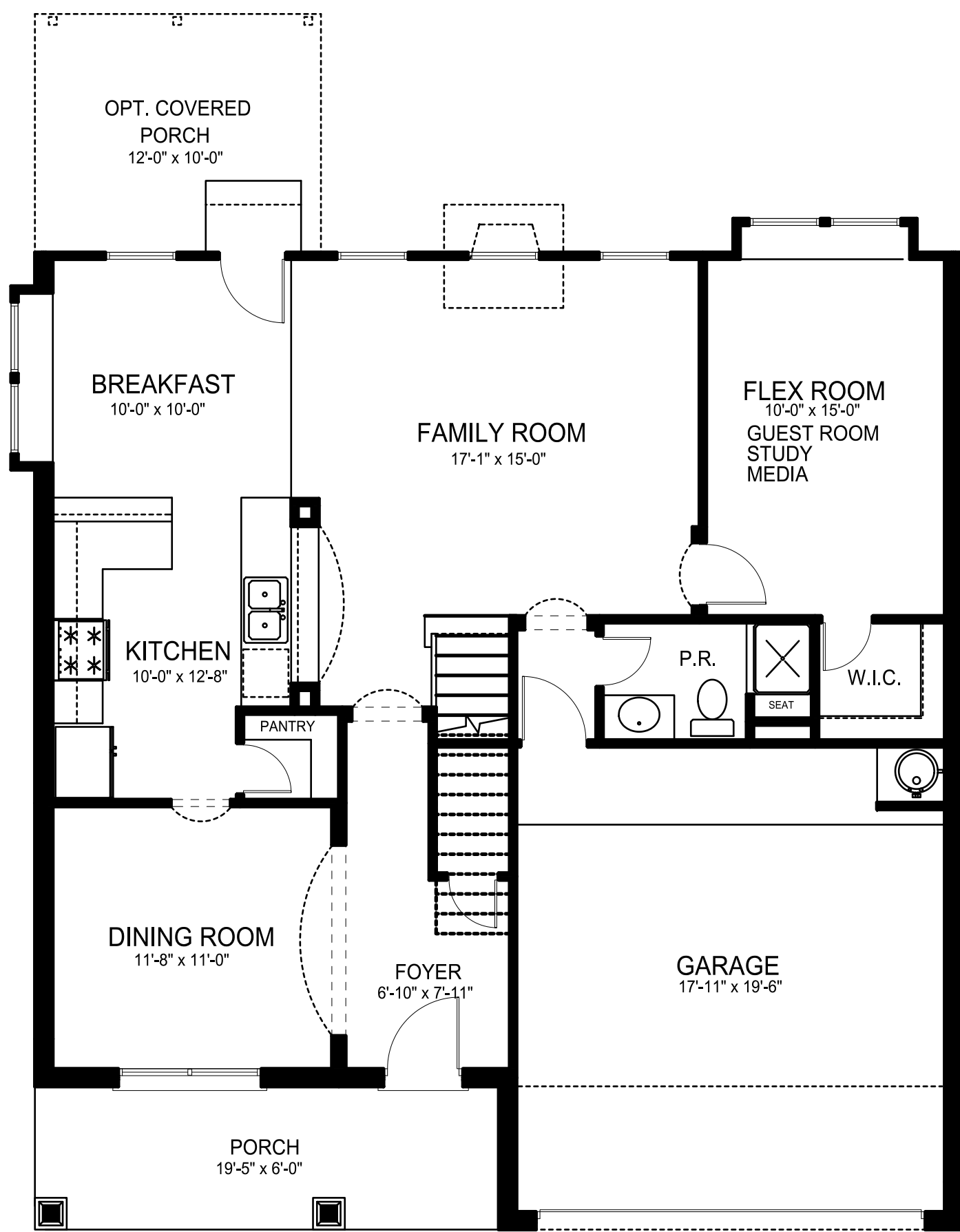
FIRST FLOOR
