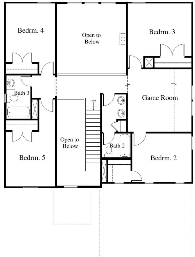
SECOND FLOOR PLAN D
